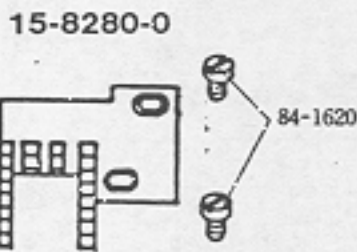
Presser foot (2 Needles)
