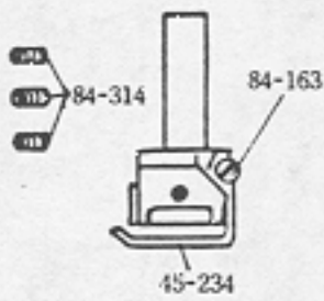
Needle holder (2,3 Needles)
