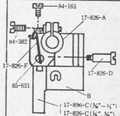
Needle plate (2 Needles)
