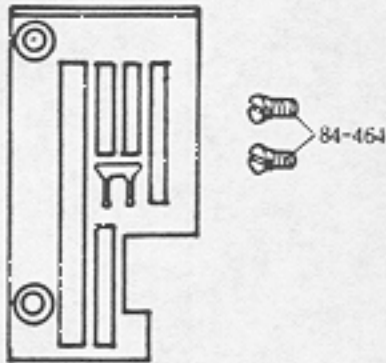
Needle plate (2 Needles)
