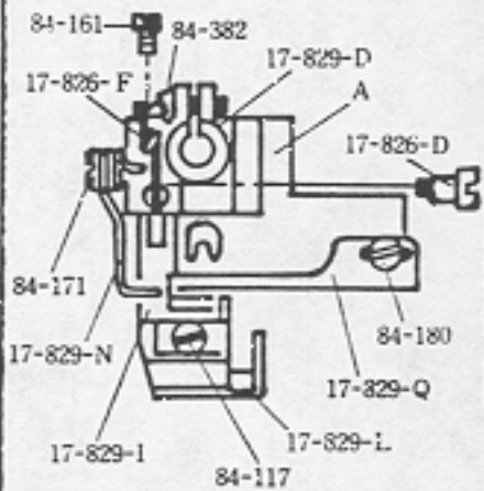
Presser foot (2 Needles)
