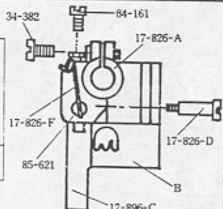
Needle plate (3 Needles)
